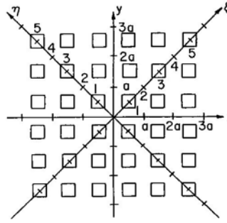
Fig. 4. Rotated and rescaled coordinate system used for performing the integration of the spatial power spectral density. The side of each square is \nu
