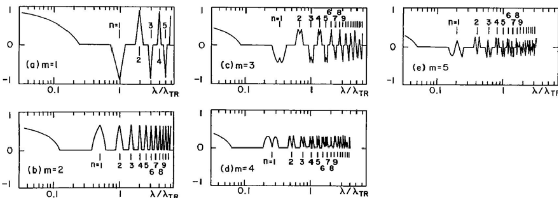
Fig. 5a-e. The dependence of the various spatial power spectrum Fourier coefficients on \lambda/\lambda_{TR} at N = \infty . Geometry ( R_1 = R_2 = 0.5 , a = 10^{-5} , \tilde{x}_2/a = 1/4 , \lambda_{TR} = 4 \times 10^{-10} , unit transmission slits) is held fixed while wavelength is varied, thereby displaying the finite-width resonance phenomena. a through e display, respectively, harmonic #1 (fundamental) showing m = 1 resonances through harmonic #5 showing m = 5 resonances. Tics mark associated n value at \lambda/\lambda_{TR} = n/m .
