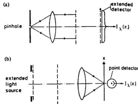
Fig. 8. a Diagram of Talbot's apparatus. b Diagram of von Lau's apparatus. (Figures after Jahns and Lohmann)
