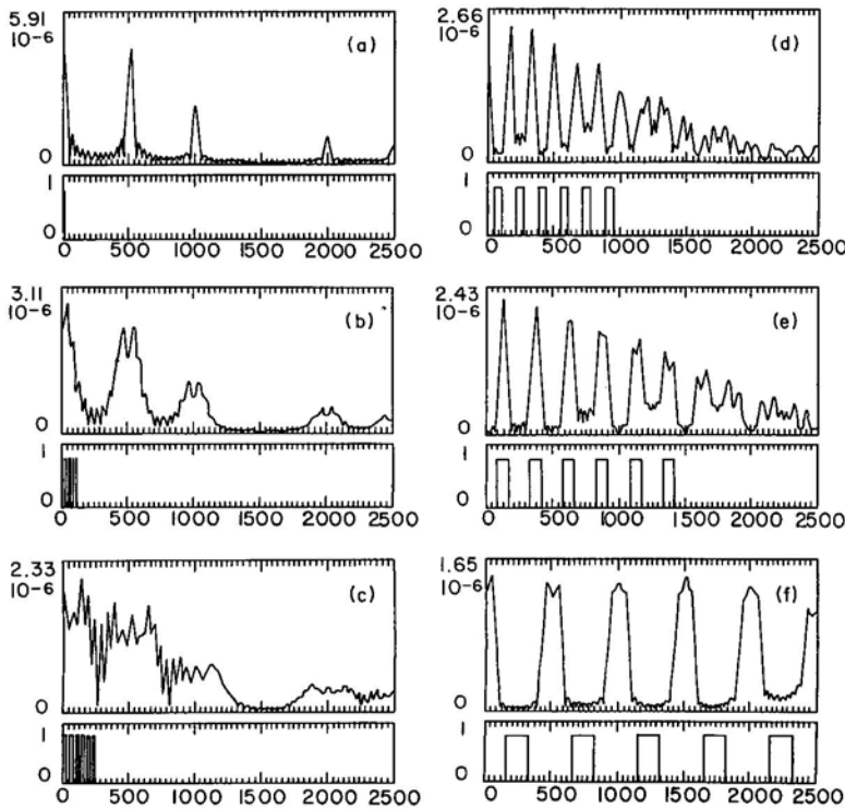
Fig. 3a–f. Image intensity and associated geometric shadow patterns (symmetric about the origin, horizontal-axis = \tilde{x}_2 , in units = 10^{-6} ) showing the transition from Fraunhofer diffraction orders to generalized Talbot-von Lau fringes for various R_1 and for a grating with N = 12 slits, s/a = 1/3 , R_2 = 1 , a = 10^{-6} , and fixed \lambda = 0.5 \times 10^{-9} . Fraunhofer orders occur at the major horizontal-axis divisions, i.e., at integral multiples of 500 \times 10^{-6} , while the horizontal-axis subdivisions are at the order spacing N . a has R_1 = \infty , \mu/n = 0.002 , and (49) satisfied. b has R_1 = 0.0504 , \mu/n = 1/24 , and (49) an equality. c has R_1 = 0.0246 , \mu/n = 1/12 , (49) violated. d–f correspond to cases with \mu = m = 1 , with (52) violated and with n = 3 ( R_1 = 0.006 ), n = 2 ( R_1 = 0.004 ), and n = 1 ( R_1 = 0.002 ), respectively
