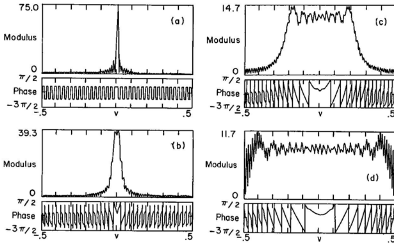
Fig. 2a-d. Numerical evaluation of the modulus and phase of one period of P(v) as a function of v for various values of \epsilon for n = 1 and r = N = 75 . a \epsilon = 0 , b \epsilon = 1/(16N) , c \epsilon = 1/(2N) , d \epsilon = 1/N
